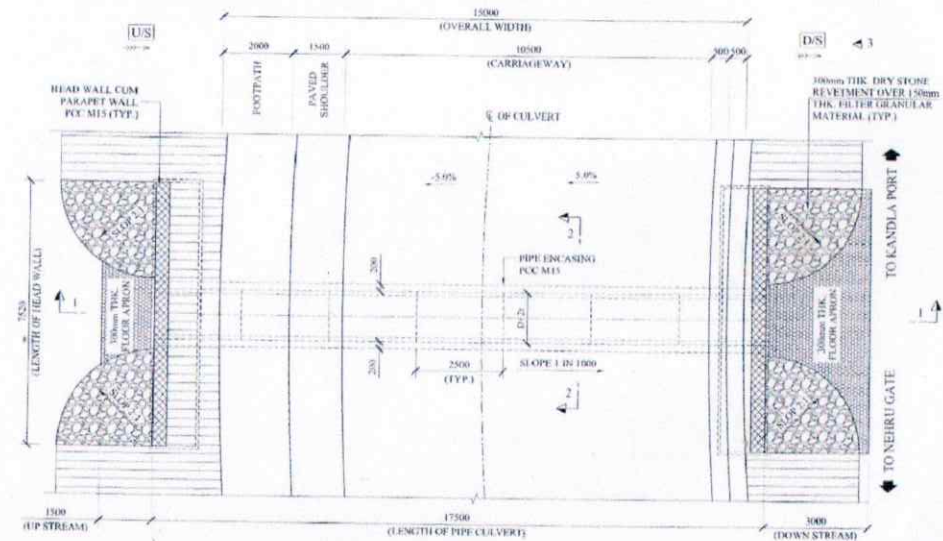
PLAN (SCALE 1:100)
