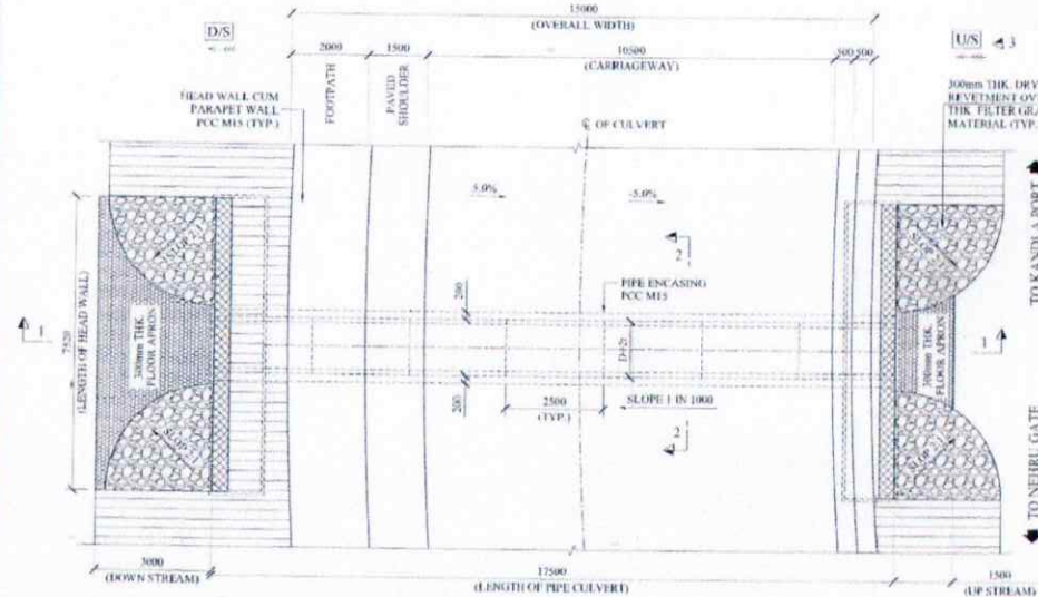
PLAN (SCALE 1:100)
