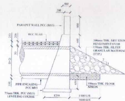
DETAIL-A (SEE FIG. 1-50)
