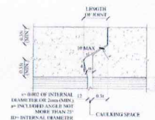
DETAIL-B INTERNAL JOINT (SCALE 1:4)
