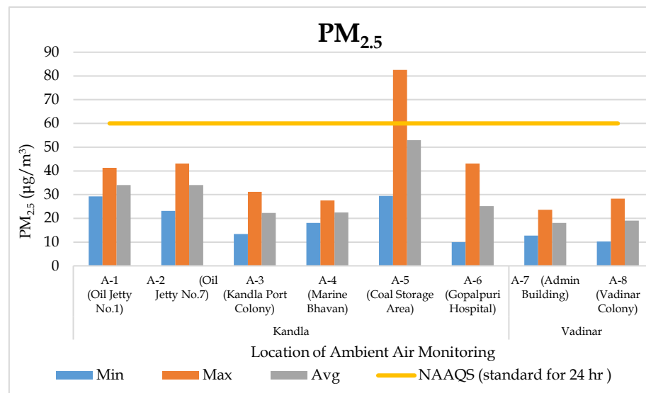
Graph 2: Spatial trend in Ambient PM 2.5 Concentration
