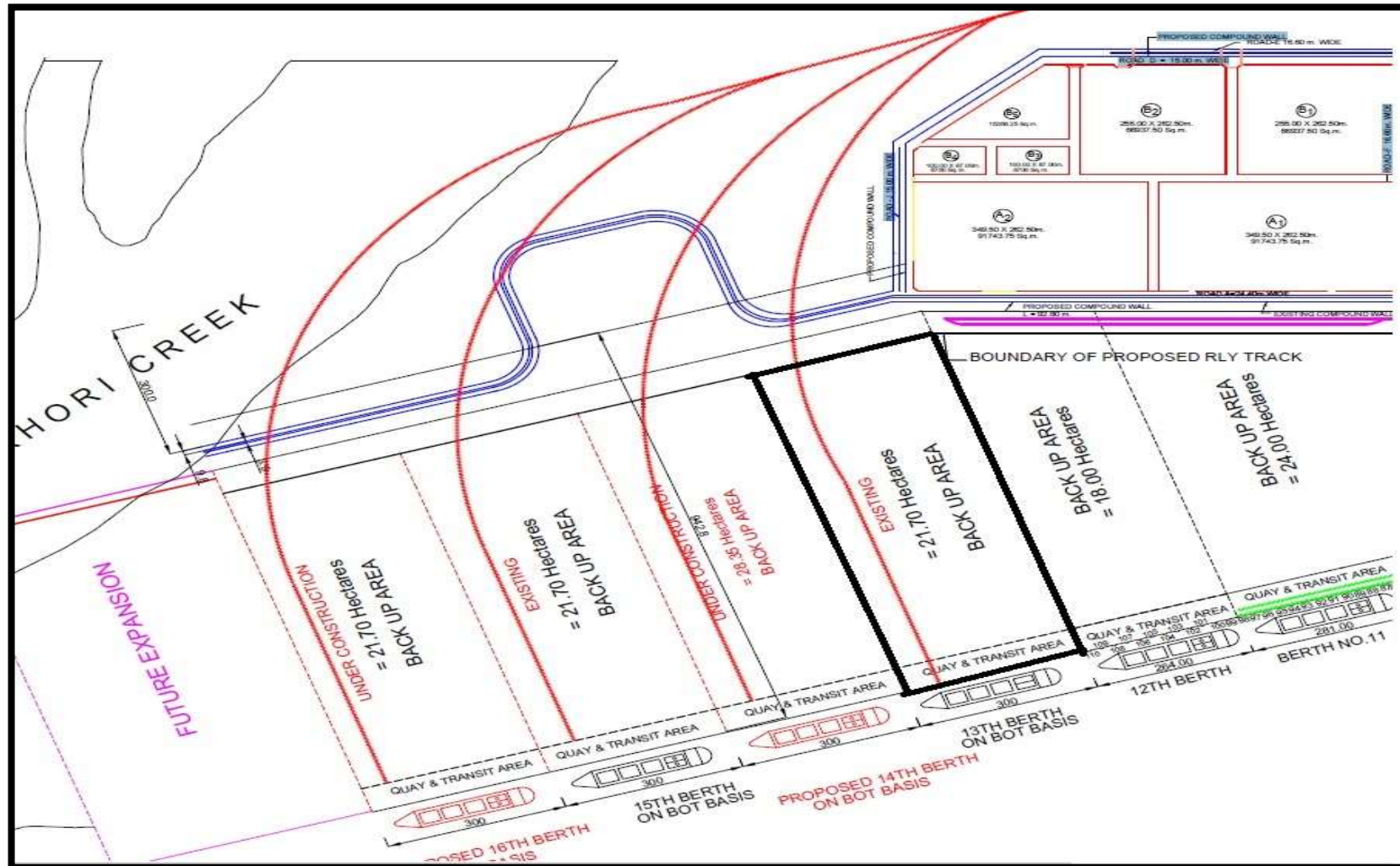
Berth-13 Layout
